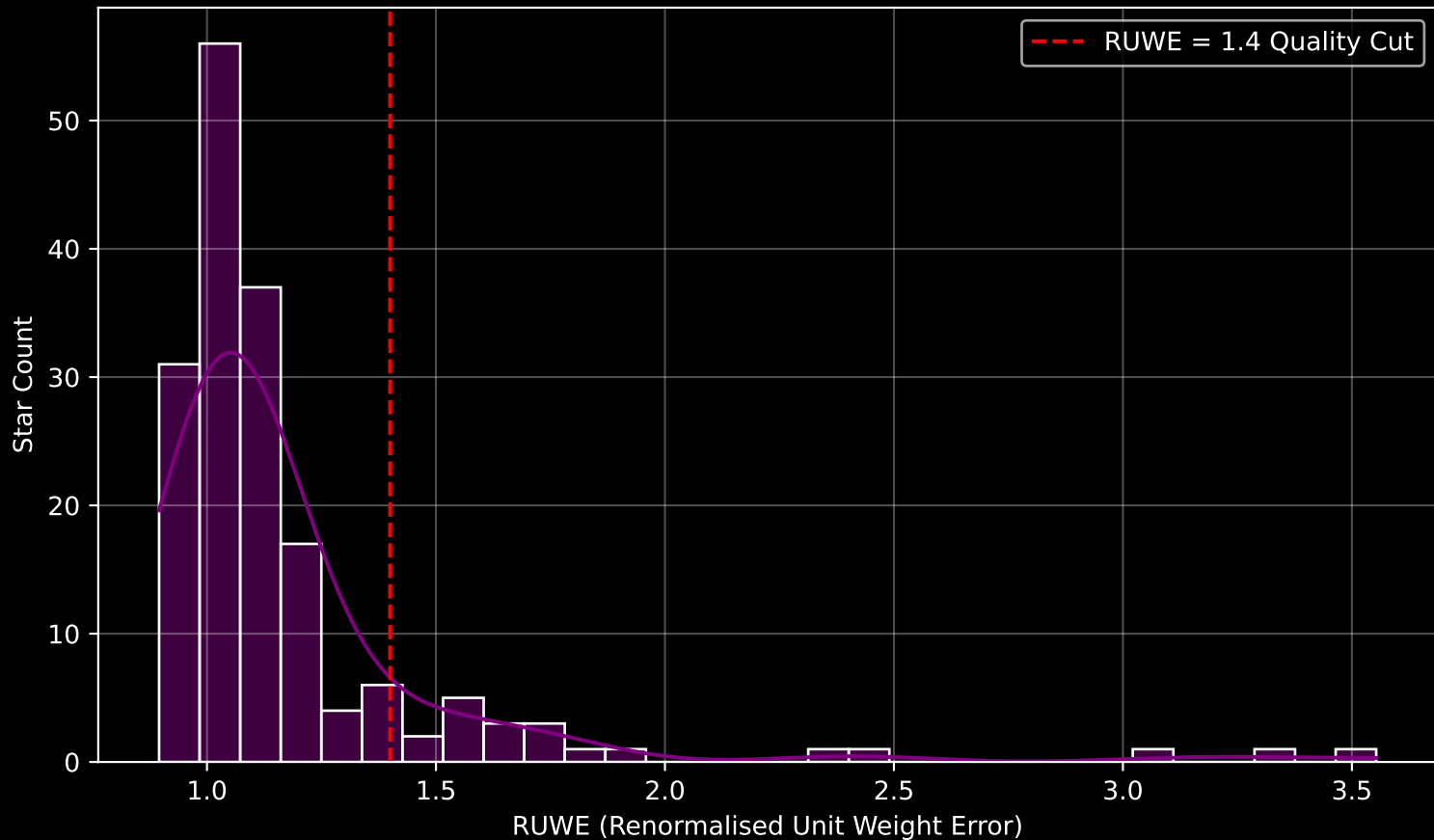
GALAH DR4 Field [208] RUWE Distribution (n= 171)
