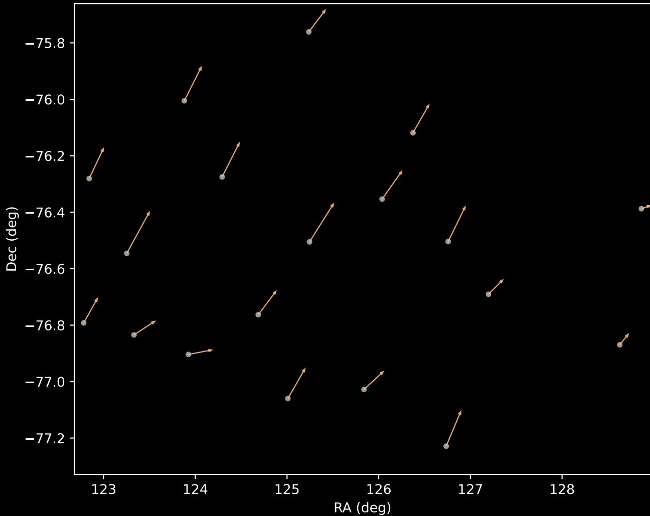
GALAH DR4 Cluster 3 Proper Motion Vectors (n=19)
