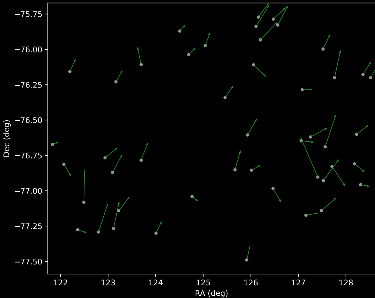
GALAH DR4 Cluster 4 Proper Motion Vectors (n=46)
