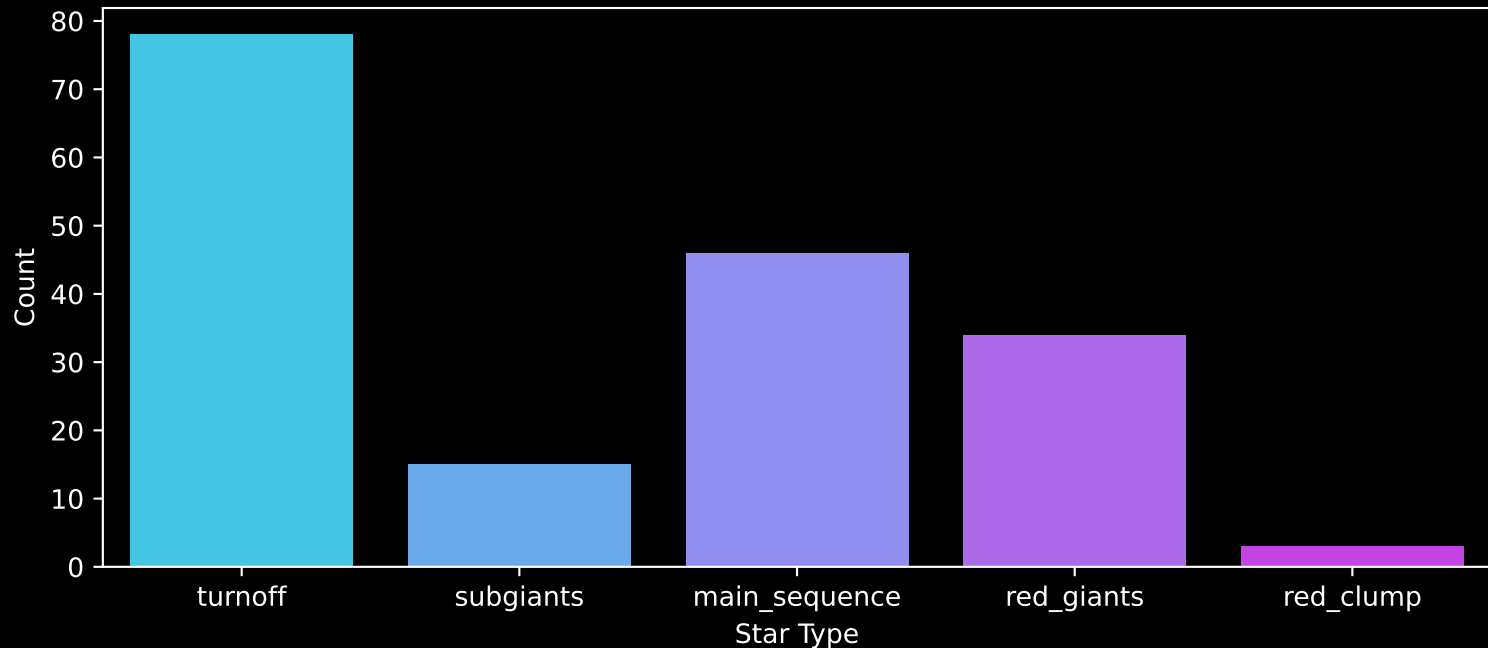
GALAH DR4 Field: [208] Count plot of Star Type
